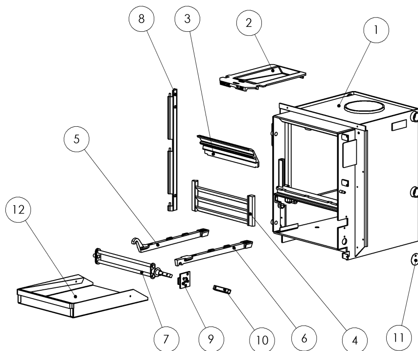
BOILER BODY ASSEMBLY
